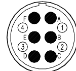
FACE VIEW PIN CONNECTOR
